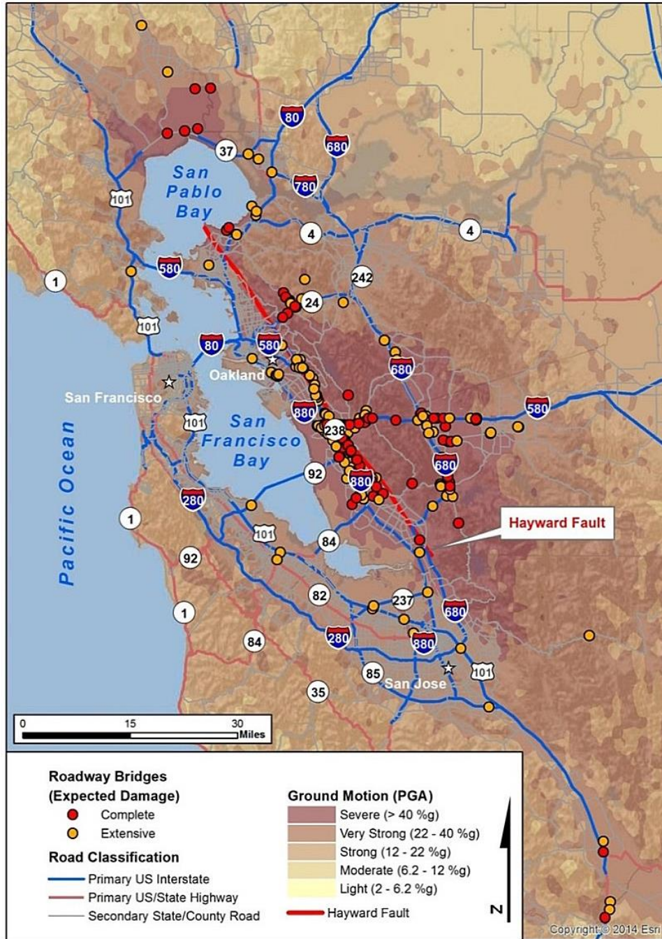
FIGURE 5—AFFECTED ROADWAY BRIDGES, COMPLETE OR EXTENSIVE EXPECTED DAMAGE STATES
